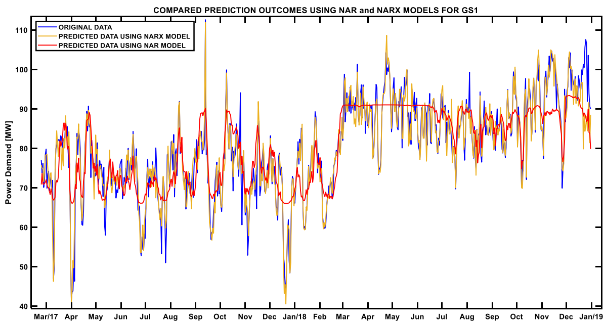
Fig. 4. Comparison between the observed and the predicted power demand values from the NAR and NARX models for the GS1 site. The climate variables are only considered as exogenous inputs in the NARX model.
