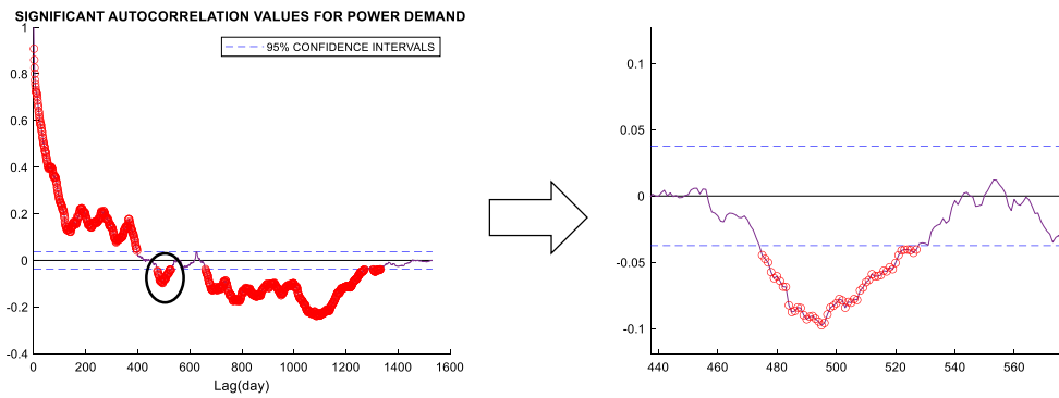
Fig. 3. Autocorrelation result of input data and the red circle is the significant points or values which is used as FD in the training process.
