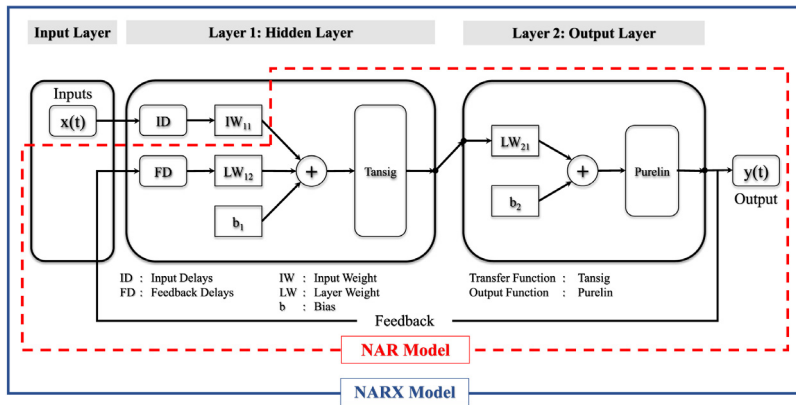
Fig. 2. Structure of the NAR and NARX model. The NAR model has no exogenous inputs (red boundary), whereas the NARX model includes exogenous inputs (climate variables) for improving the predicting models (blue border).
